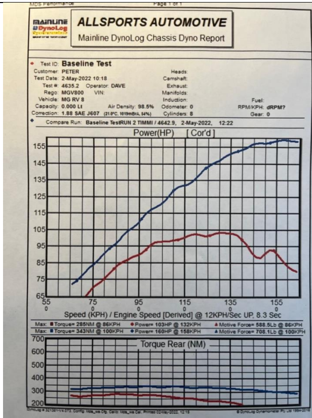
Figure 7 Dyno tuning
